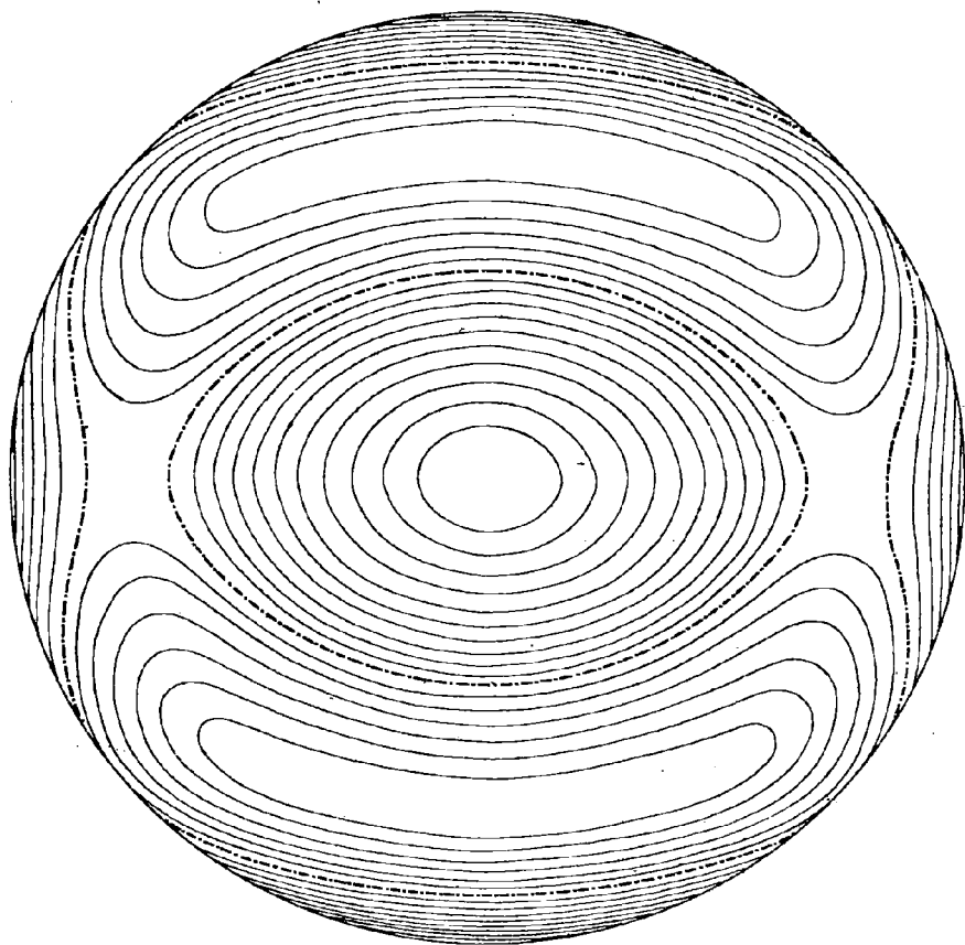
Spherical Harmonic of the fourth degree.
