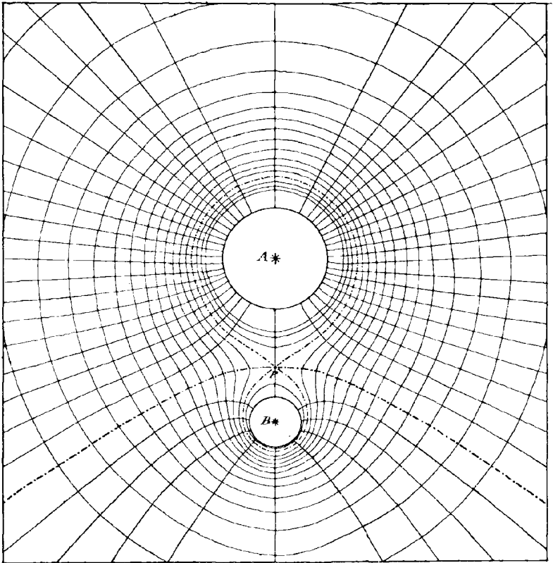
Lines of Force and Equipotential Surfaces.
