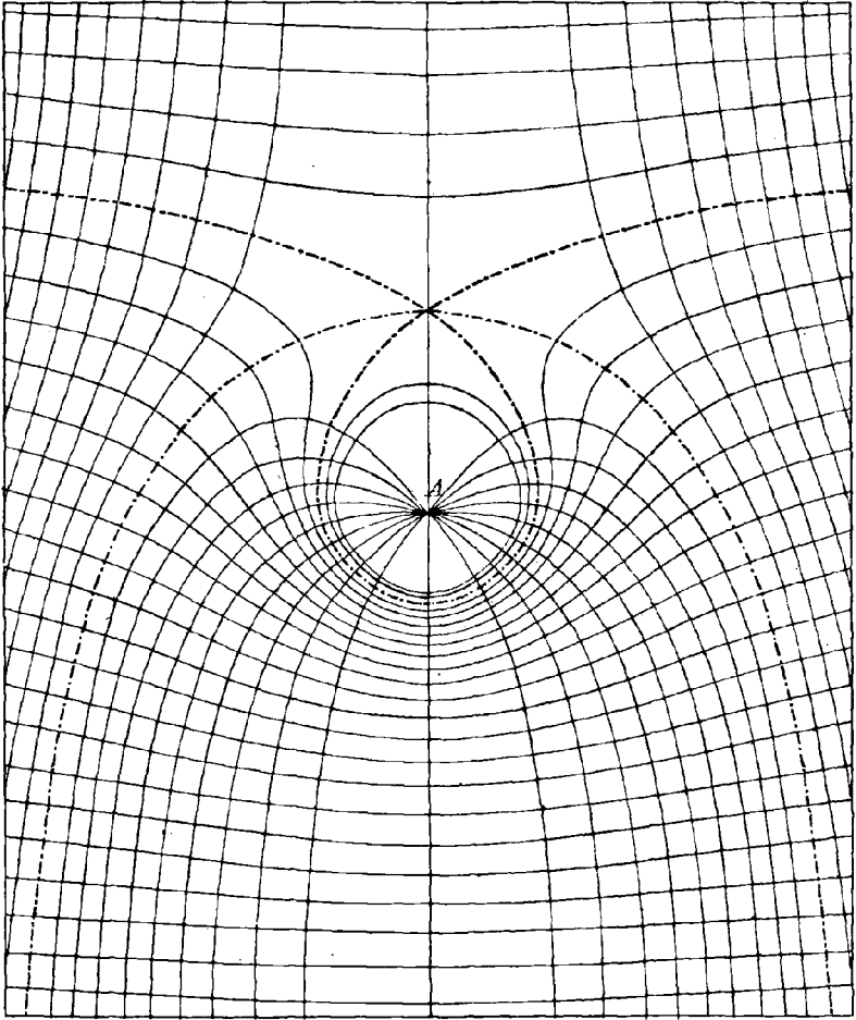
Lines of Force and Equipotential Surfaces.
