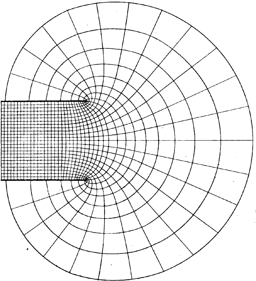
Lines of Force between two Plates.
