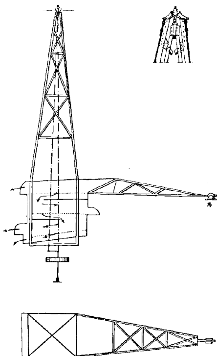
FIG. 10. — Crible Kartick.
