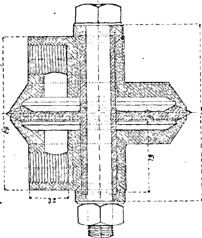
FIG. 58. — Appareil Bereznef.
