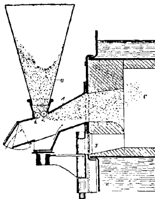
FIG. 51. — Foyer Pinther.
