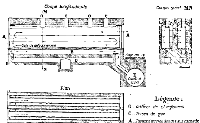
FIG. 176. — Four Semet-Solvay.
