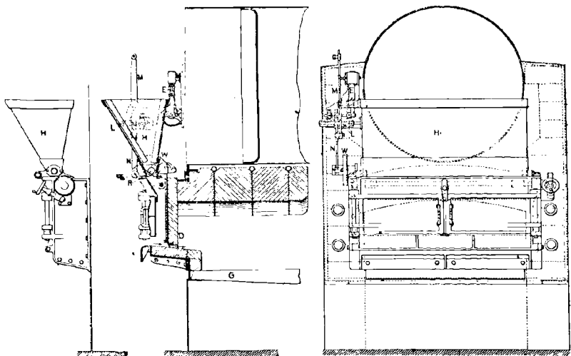
FIG. 50. — Foyer Westlake.
