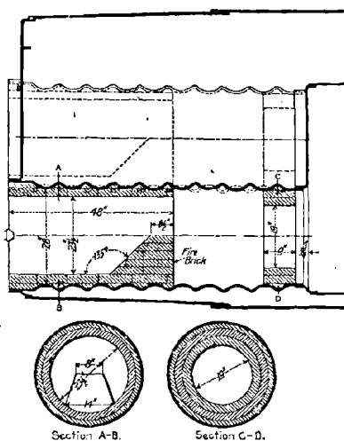
FIG. 91, 92, 93. — Foyer Player.
