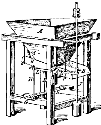
FIG. 44. — Tulloch's ore feeder 1 .
