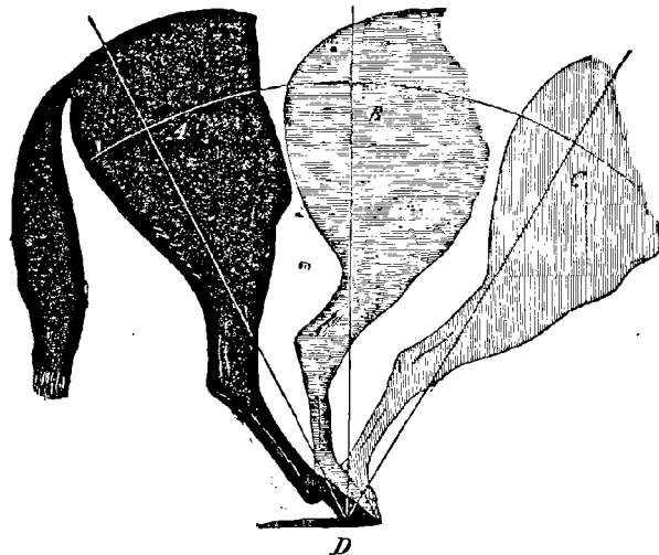
Fig. 160. Force impulsive.
