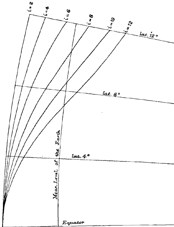
FIG. 3. Diagram showing the profile of the even harmonics near the Equator. Radius of sphere 18 inches.
