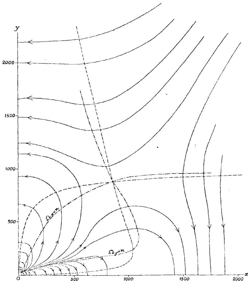
FIG. 2. Lines of greatest slope on the surface 2z = (3 - x^{\frac{1}{2}} - 2y^{\frac{1}{2}})^2 - 20 \left( \frac{1}{x^{\frac{1}{2}}} + \frac{2}{y^{\frac{1}{2}}} \right) .
