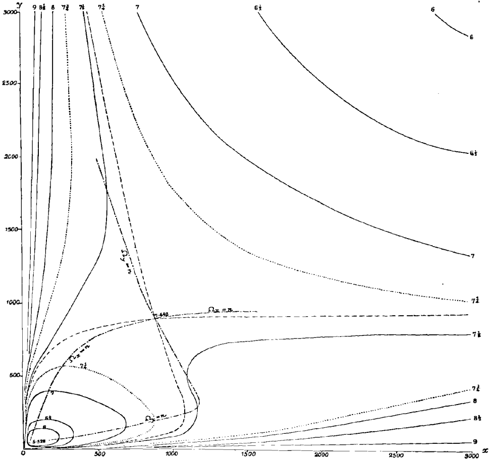
FIG. 1. Contours of the surface 2z = (9 - x^{1/2} - 2y^{1/2})^2 - 20\left(\frac{1}{x^{1/2}} + \frac{2}{y^{1/2}}\right) when x and y are both positive.
