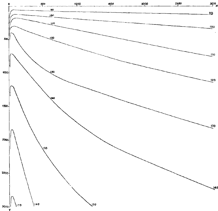
Fig. 5. Contour lines of the surface 2z = (9 - x^{1/2} - 2y^{1/2})^2 - 20 \left( \frac{1}{x^{3/2}} + \frac{2}{y^{3/2}} \right) when x is positive and y negative.
