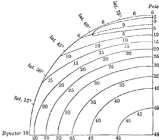
FIG. 1. Diagram showing surfaces of equal stress-difference due to the weight of second harmonic inequalities or to tide-generating force.
