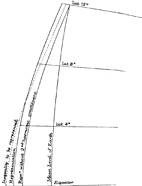
FIG. 5. Diagram showing the profile of isolated equatorial continents. Radius of sphere 18 inches.
