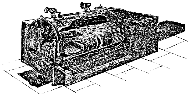
Fig. 40. — Chaudière Galloway compound.
