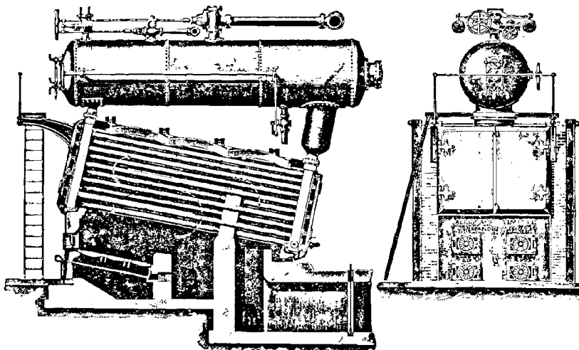
Fig. 44. — Chaudière Manchester.
